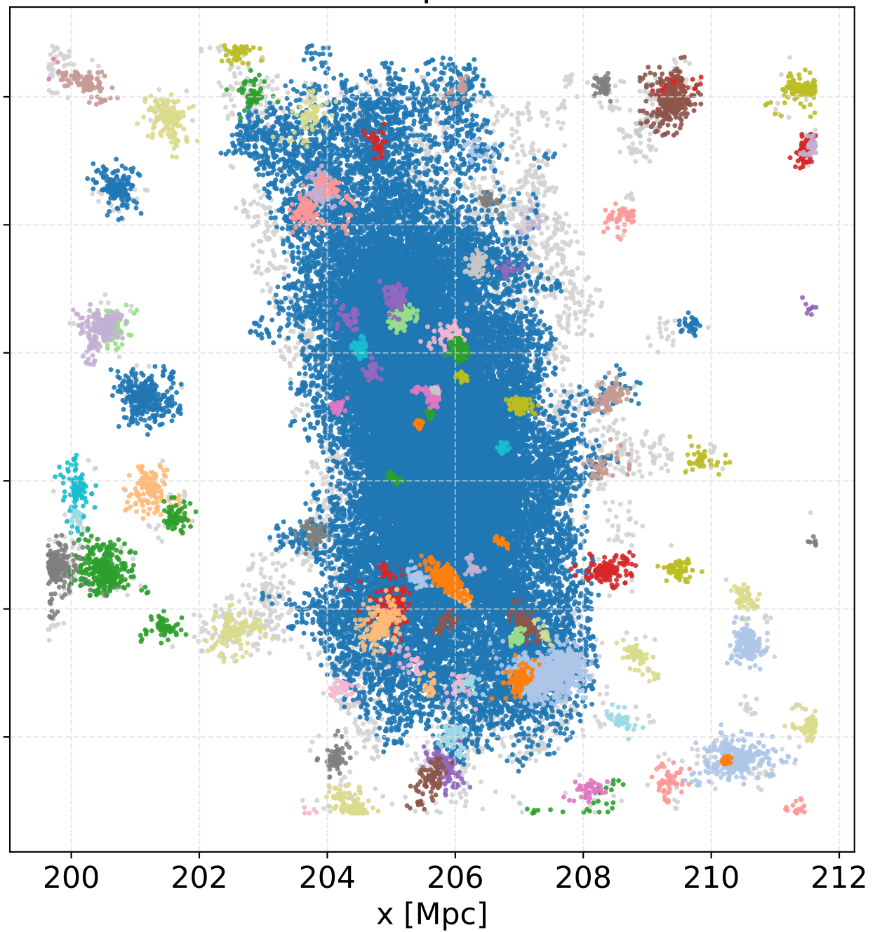
HALOS particles
